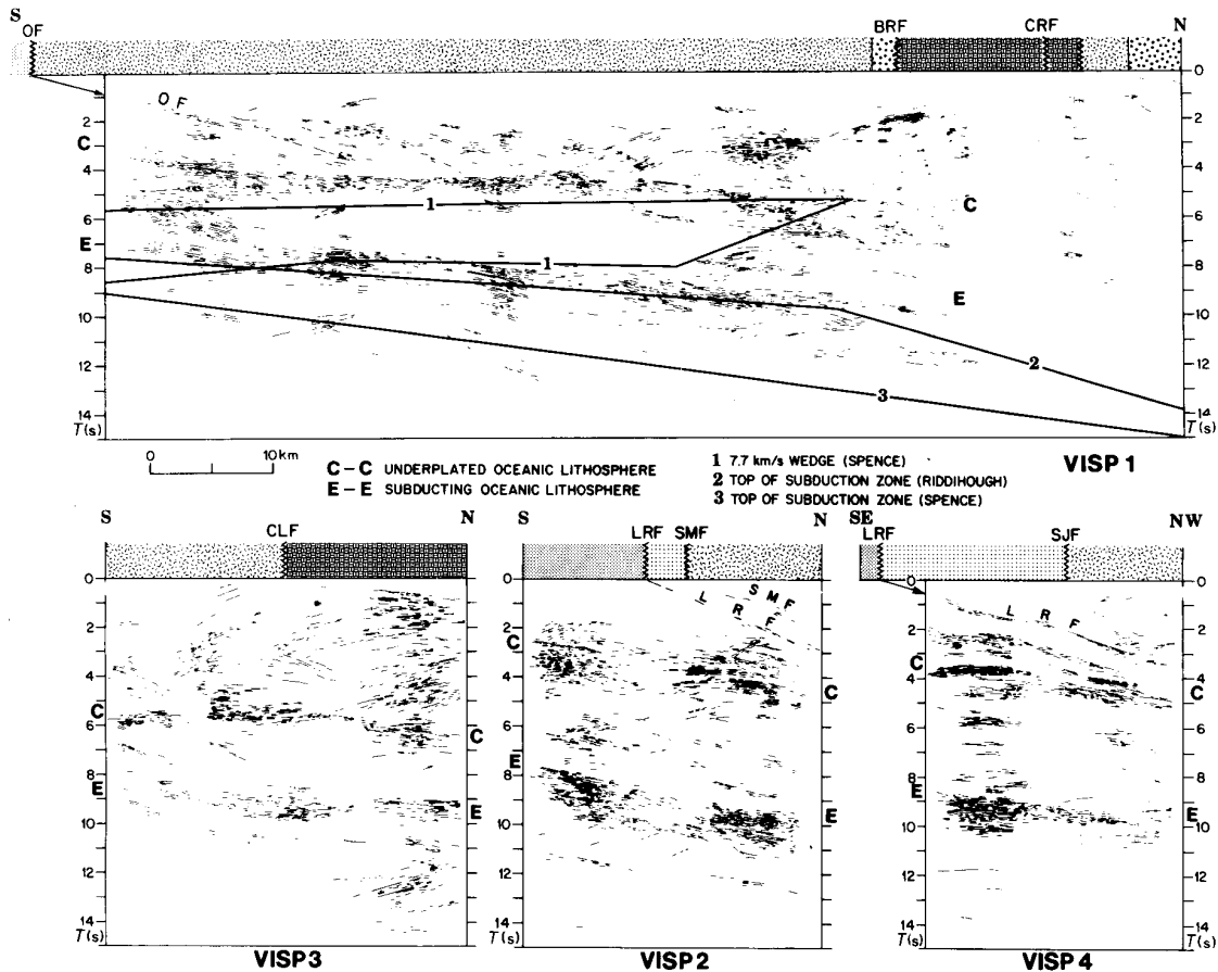
Fig. 2 Line drawings showing the unmigrated reflections recorded on the four seismic reflection profiles. Vertical scale is two-way travel-time in seconds ( T ). All lines were recorded to 16 s with 30-fold coverage. Acquisition methods were similar to those used in the US by the COCORP group 45 . Final processing included single-fold trace editing, crooked line geometry and elevation corrections, automatic gain control, normal move-out corrections, trim statics using a correlation window of T = 1-12 s, common reflection point stacking, bandpass filtering of 8–40 Hz and trace-to-trace amplitude equalization using a T = 4-8 s window. Patterns at the top of each section show the surface geology crossed; an explanation of the various patterns is given in Fig. 1. On the VISPI section the -1- border delineates the high-velocity ( 7.7 \text{ km s}^{-1} ), high-density ( 3.3 \text{ g ml}^{-1} ) block proposed by Spence et al. 17 , and the -2- and -3- boundaries show, respectively, the Riddihough 10 and Spence et al. 17 estimates for the top of the actively subducting Juan de Fuca plate. C-C and E-E are prominent reflection zones that delineate the upper boundary of the high-velocity, high-density block (the underplated oceanic lithosphere) and the top of the actively subducting Juan de Fuca plate respectively. OF, Offshore (or Tofino 46 ) Fault; BRF, Beaufort Range Fault; CRF, Cameron River Fault; CLF, Cowichan Lake Fault; LRF, Leech River Fault; SMF, Survey Mountain Fault; SJF, San Juan Fault (locations of faults are shown in Fig. 1). A typical example of the seismic reflection data is shown in Fig. 3.
