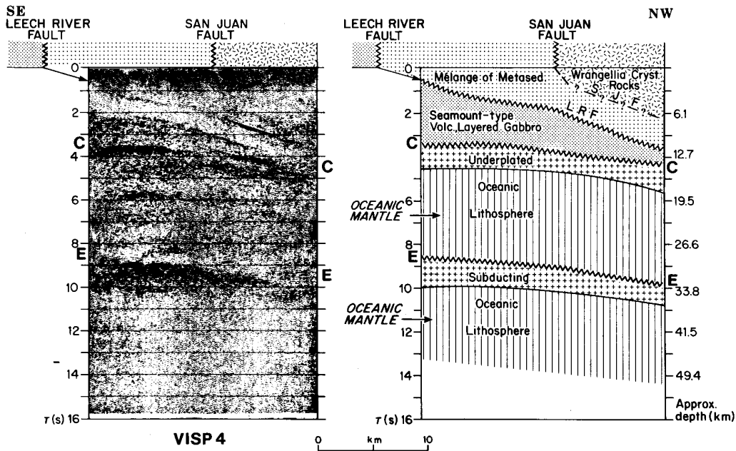
Fig. 3 A typical unmigrated seismic reflection section and simplified interpretation obtained from data recorded on Vancouver Island. Figure 1 shows the location of the profile and Fig. 2 (bottom right) shows a line diagram of the individual reflections recorded on the section. Patterns at the top of both the section and the interpretation diagram show the surface geology; an explanation of the various patterns is given in Fig. 1. The regions of + signs correspond to the reflection zones C and E. Approximate depths shown are based on the seismic refraction model of Spence et al. 17 . The seismic reflection data were recorded by Veritas Geophysical Ltd and processed by Veritas Seismic Ltd.
