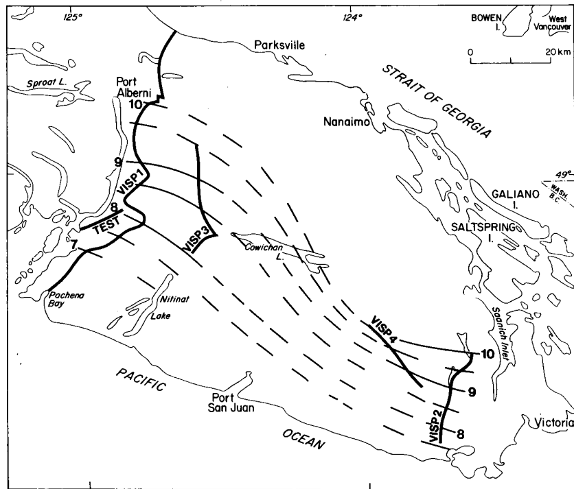
Fig. 4 Contours are two-way travel-times (unmigrated) (in s) to the top of reflection zone E. The curvature of the dashed contours between the western pair of seismic profiles (VISP1 and VISP3) and the eastern pair (VISP2 and VISP4) is speculative; a major fault anywhere between the two pairs of profiles would be an equally valid interpretation of the travel-time information.
