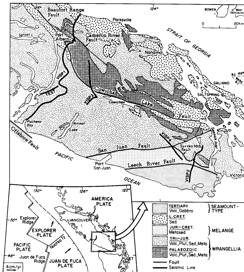
Fig. 1 Simplified geological map of southeastern Vancouver Island showing the locations of the four seismic reflection profiles, VISP1 to VISP4, and the short seismic reflection profile, TEST, of Clowes et al. 18 . Geology is mostly from Muller 44 , with minor modifications based on recent mapping programmes. The region to the north of the San Juan Fault is part of the exotic Wrangellia terrain of Palaeozoic and Mesozoic age. Between the San Juan and Leech River faults is an allochthonous mélange of Mesozoic metasediments and to the south of the Leech River Fault lies a volcanic terrain that may have been part of a Cenozoic seamount chain. The inset shows the location of the geological map with respect to the major plate boundaries.
